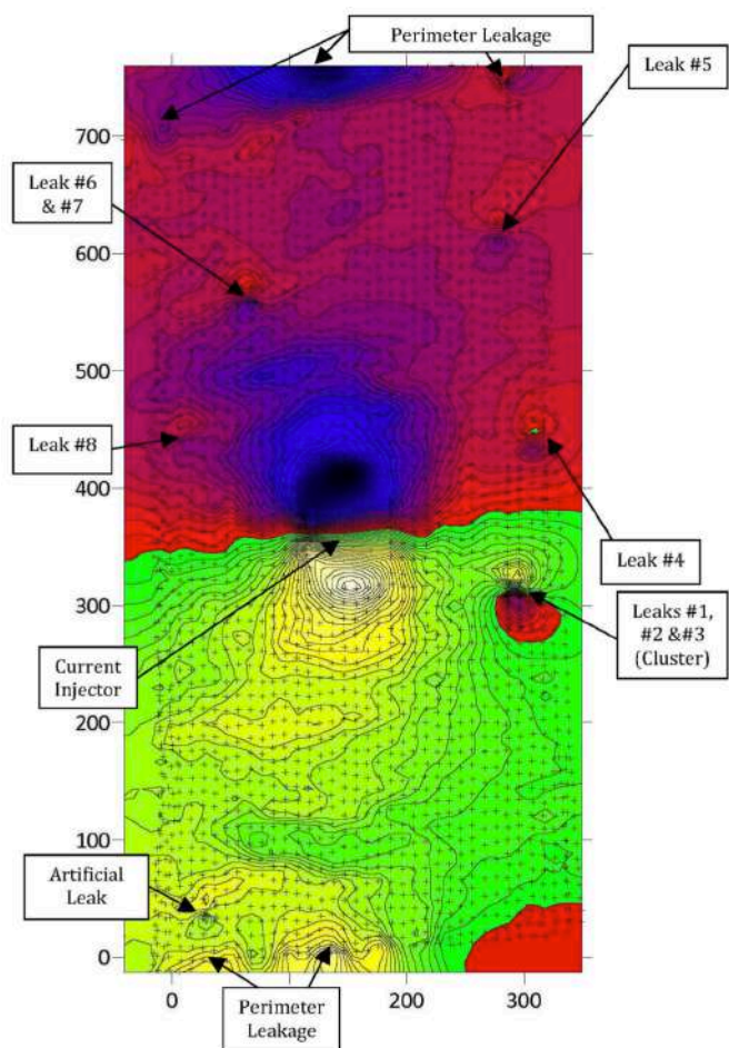
Figure 1: Example of electrical map created by dipole method ELL survey per ASTM D8265
